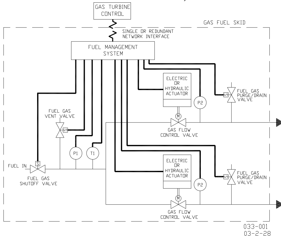
Example of a Smart Integrated Fuel System—2 Flow Path Version
